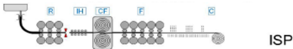
Figure 2. Schematic of In line Strip Process (ISP)
