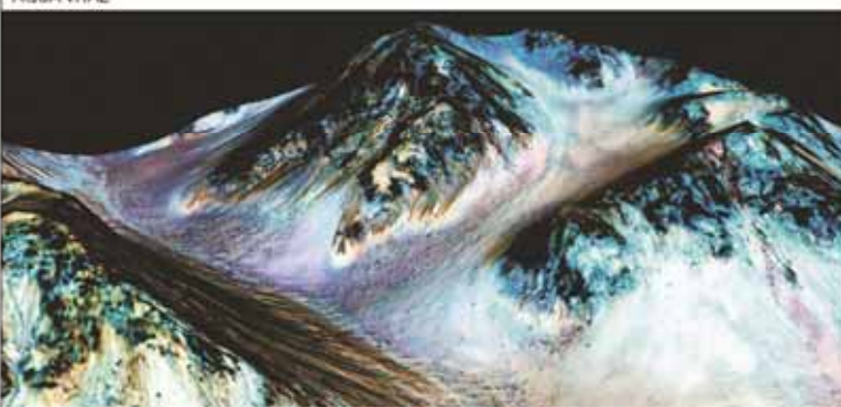
These dark, narrow, 100-meter-long streaks on Mars are believed to be evidence that water flows on the icy planet, at least during its summer. Scientists reported the finding Monday, significantly boosting the odds of life on the red planet. NASA/JPL, UNIVERSITY OF ARIZONA, AP/ISTOCK
